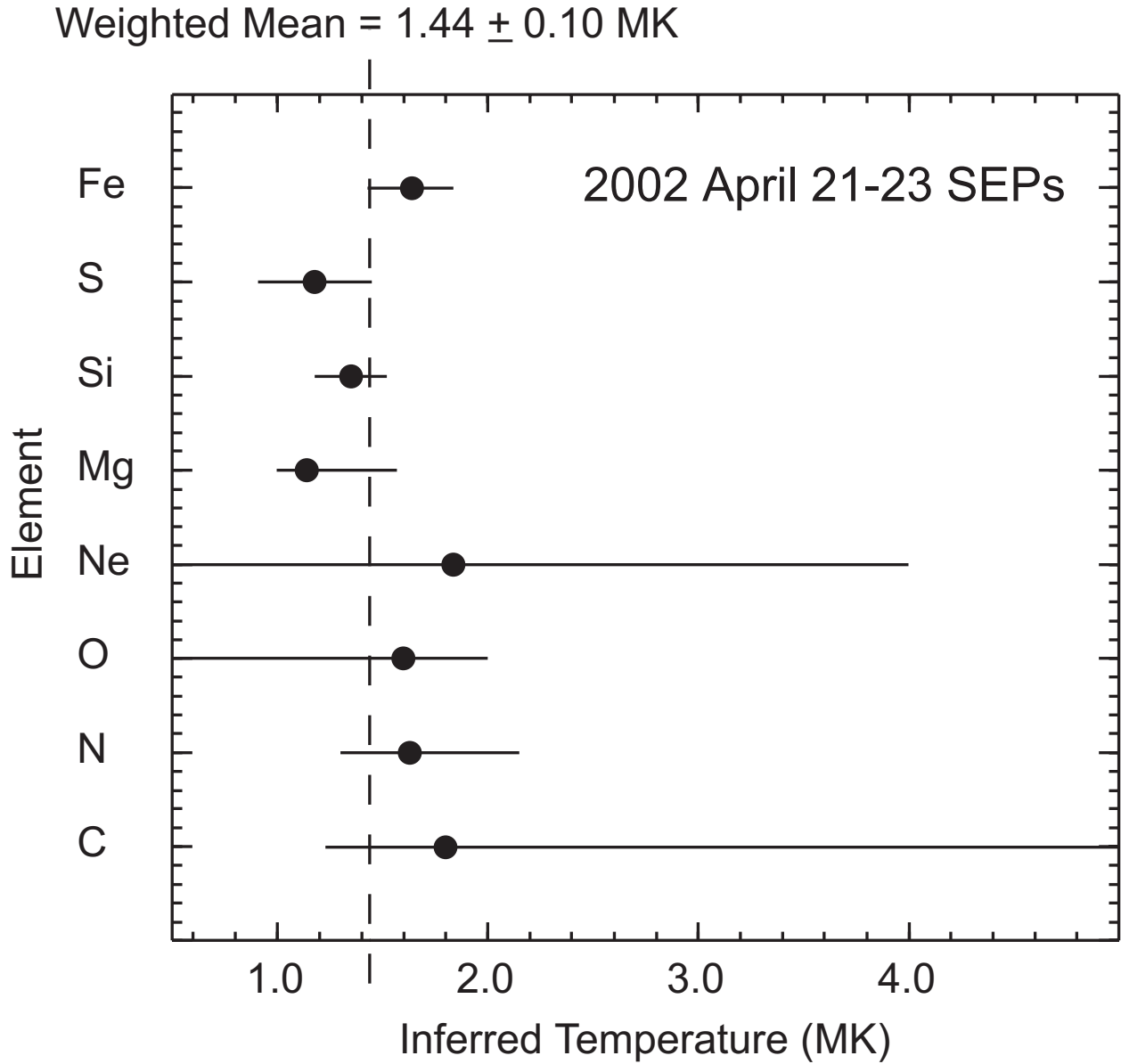
Fig. 10.— Source plasma temperatures (Arnaud & Rothenflug 1985; Arnaud & Raymond 1992), as inferred from the mean ionic charge states derived from spectral rollovers in the 2002 April 21 event.
