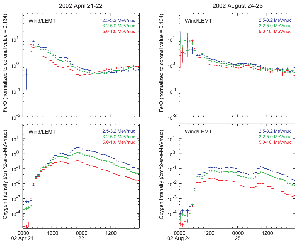
Fig. 4.— Fe/O (normalized to the nominal coronal value 0.134; top panels) and oxygen intensity (bottom panels) vs. time in the 2002 April 21 (left) and 2002 August 24 (right) events from Wind /LEMT in three energy bins covering 2.5-10 MeV/nucleon, as distinguished by colors. The datapoints are 1-hour averages.
