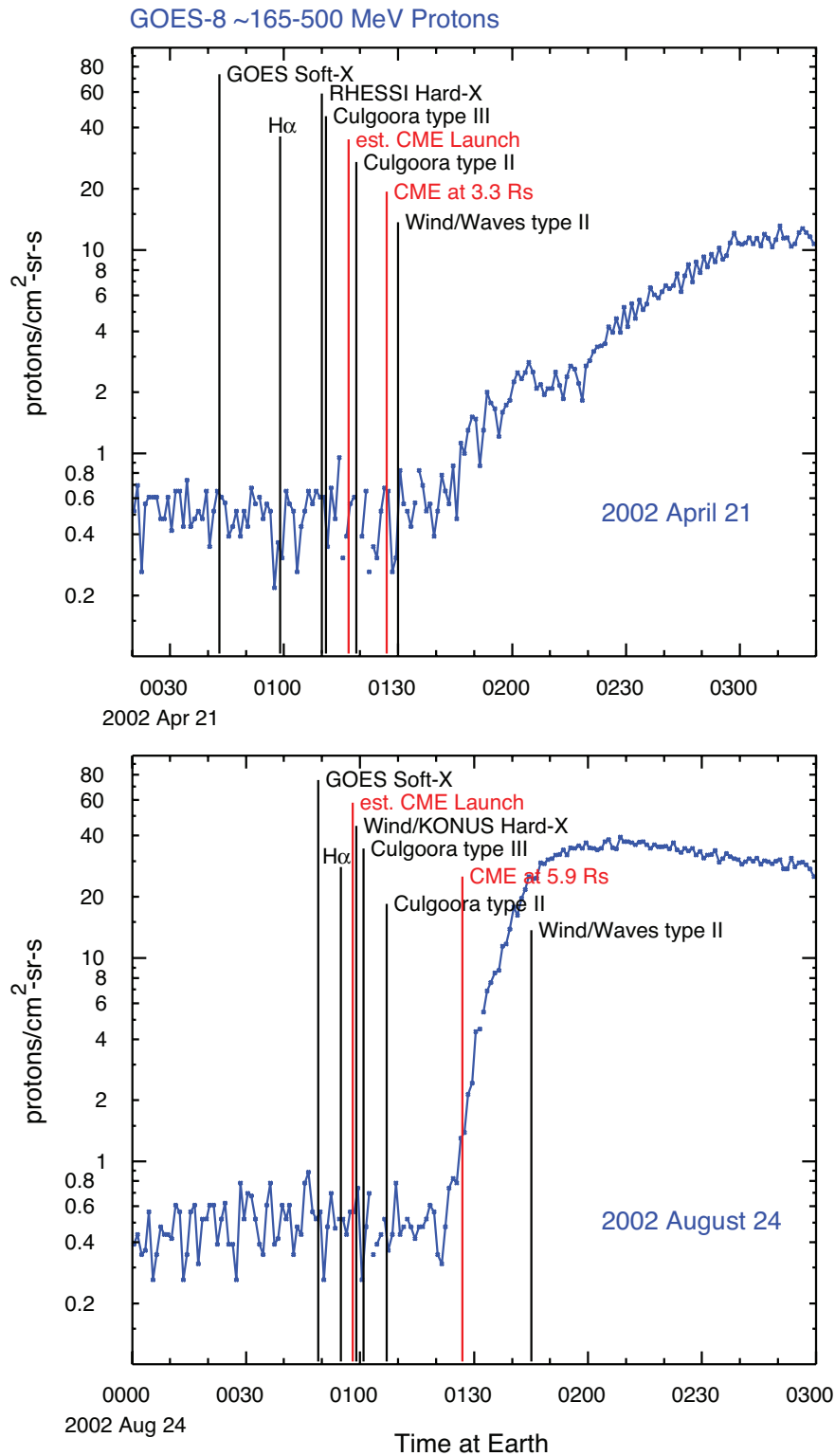
Fig. 3.— Intensities of 1-minute-averaged protons at \sim 165-500 MeV from GOES-8 over three hours spanning the start of the events on 2002 April 21 (top) and on 2002 August 24 (bottom). These are the highest-energy data for which we have high-time resolution at the onsets in both events. For comparison, black vertical lines mark the onsets of various radio and photon emissions at Earth. Red vertical lines show the time of the first LASCO CME image, as well as the estimated CME launch, as inferred from linear fits to the CME height-time profiles.
