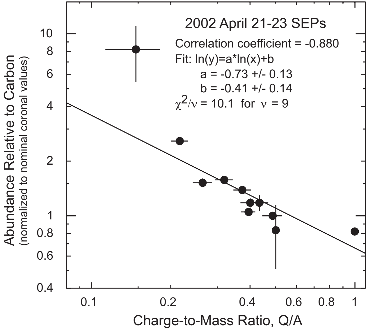
Fig. 11.— Elemental abundances relative to carbon (and normalized to nominal coronal values given by Reames (1995; 2000)) vs. charge to mass ratio (Q/A), where the charge of Z>2 elements have been taken from the spectral analysis. Also shown is a power-law fit to the correlation.
