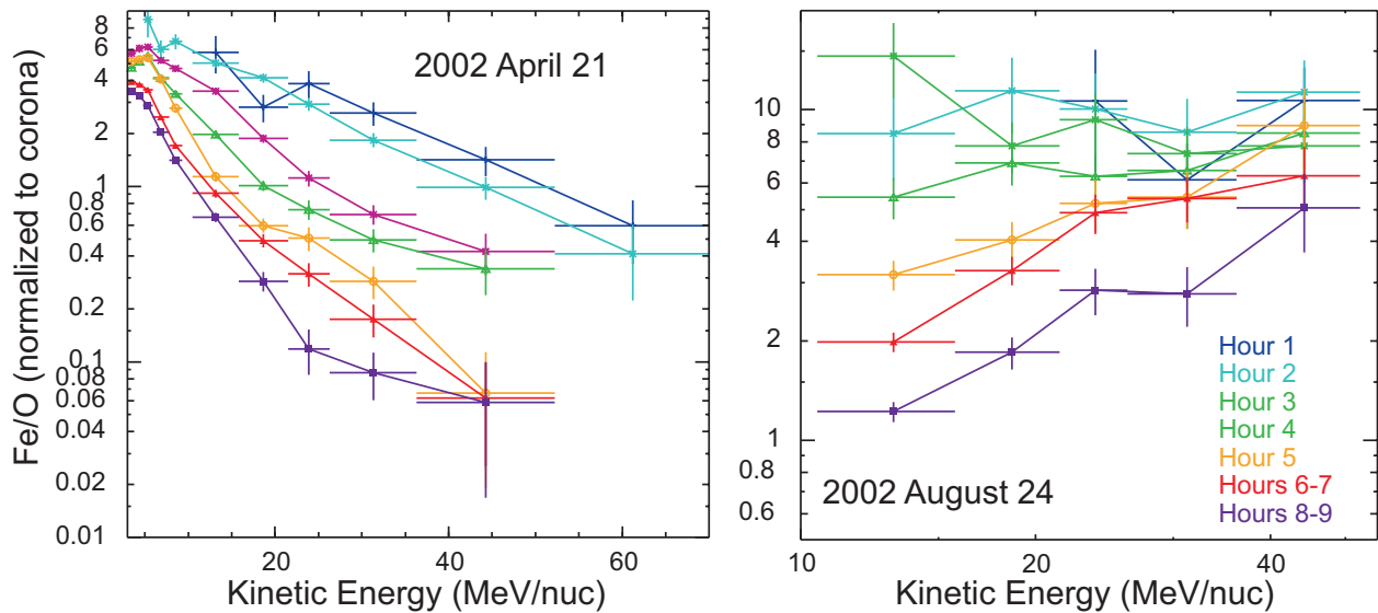
Fig. 6.— Fe/O (normalized to the nominal coronal value 0.134) vs. energy during the first nine hours of the 2002 April 21 (left) and 2002 August 24 (right) events. Time intervals are distinguished by color, as shown in the legend at the right. Datapoints below 10 MeV/nucleon are from Wind /LEMT; datapoints above 10 MeV/nucleon are from ACE /SIS. Note the difference in the vertical scale on the two panels. The left panel is log-linear, so as to emphasize the nearly exponential drop in Fe/O with energy in the April event. The right panel is log-log, showing that after the first three hours of the August event, Fe/O above 10 MeV/nucleon increases with energy roughly as a power-law.
