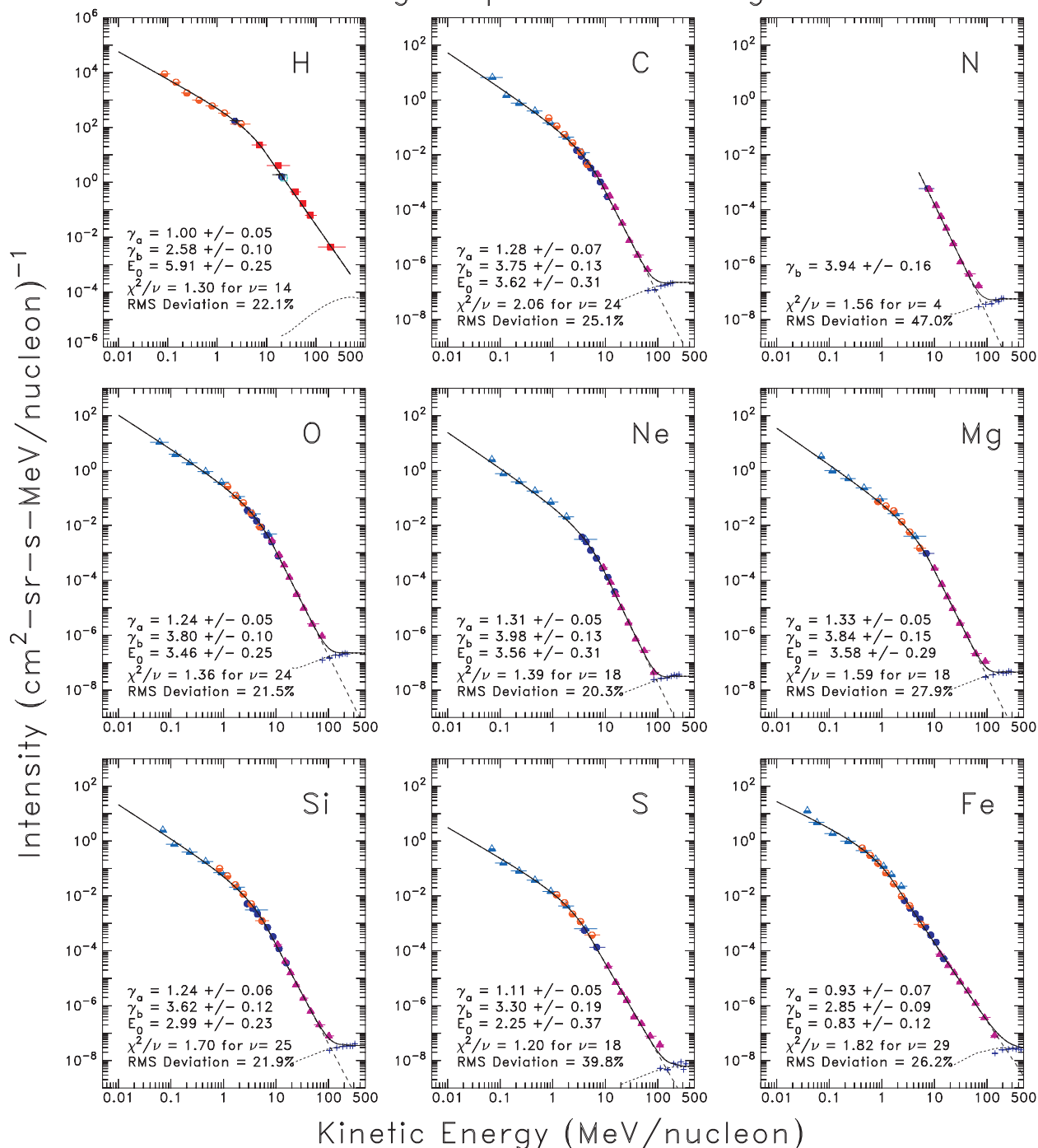
Fig. 13.— Event-averaged spectra for the major elements in the 2002 August 24 solar particle event. The averaging interval began at 0:00 UT on 2002 August 24 and ended at 0:00 UT on 2002 August 27. Instruments are distinguished by color and symbol, as in Figure 7. Fits are to Band et al. (1993) functions, as described in the text. Fit parameters, reduced \chi^2 , and rms deviation of the residuals are noted in each panel.
