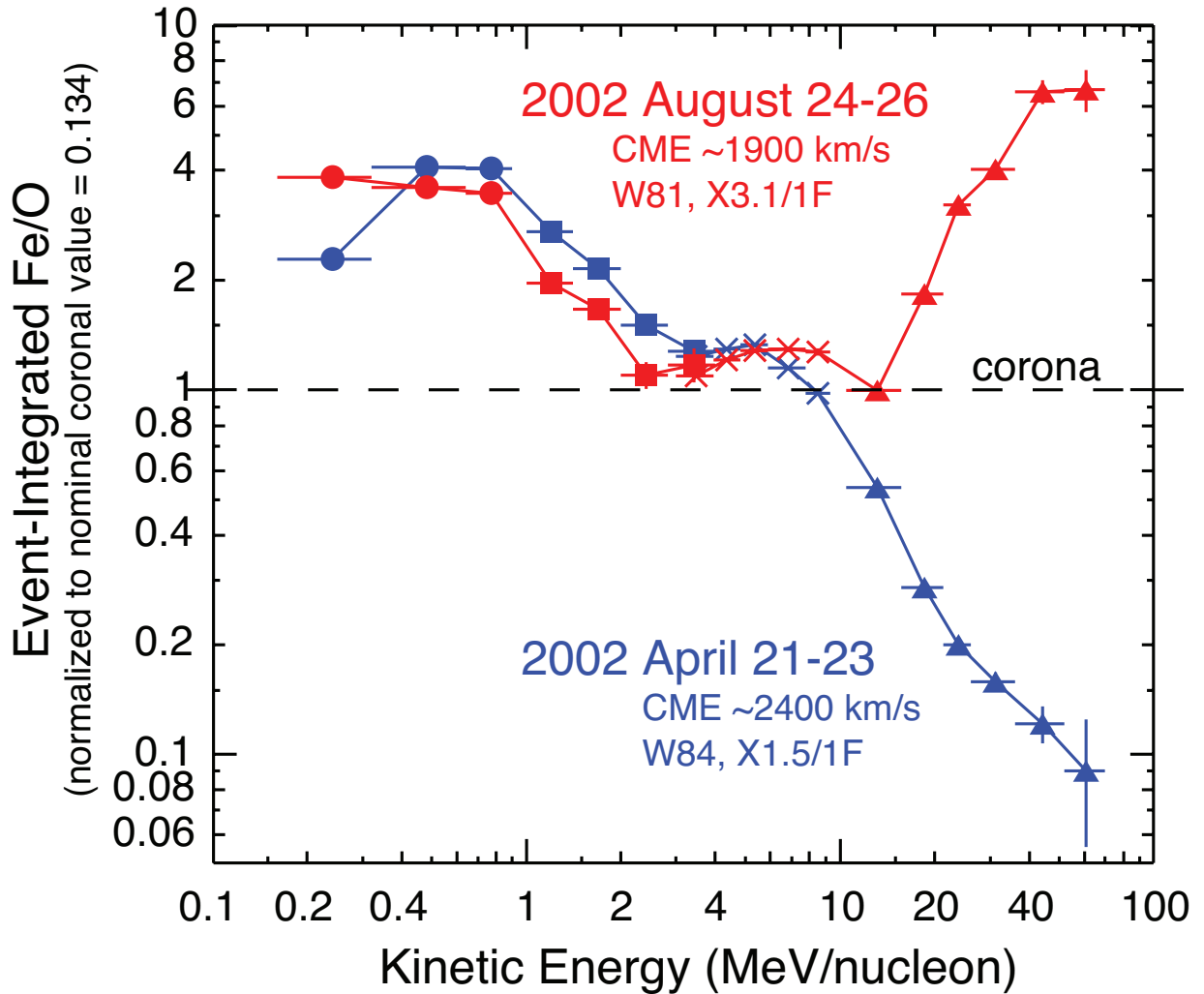
Fig. 1.— Event-integrated Fe/O (normalized to the nominal coronal value 0.134 (Reames 1995)) versus energy for the solar energetic particle (SEP) events of 2002 April 21 (blue) and 2002 August 24 (red). In both events, the event integration was for 72 hours. Data come from the Ultra Low-Energy Isotope Spectrometer (ULEIS; Mason et al. 1998; filled circles) on the Advanced Composition Explorer ( ACE ), the Electron Proton, and Alpha Monitor (EPAM; Gold et al. 1999; filled squares) on ACE , the Low Energy Matrix Telescope (LEMT) in the Energetic Particle Acceleration, Composition, and Transport (EPACT) experiment (von Rosenvinge et al. 1995; crosses) on Wind , and the Solar Isotope Spectrometer (SIS; Stone et al. 1998a; filled triangles) on ACE .
