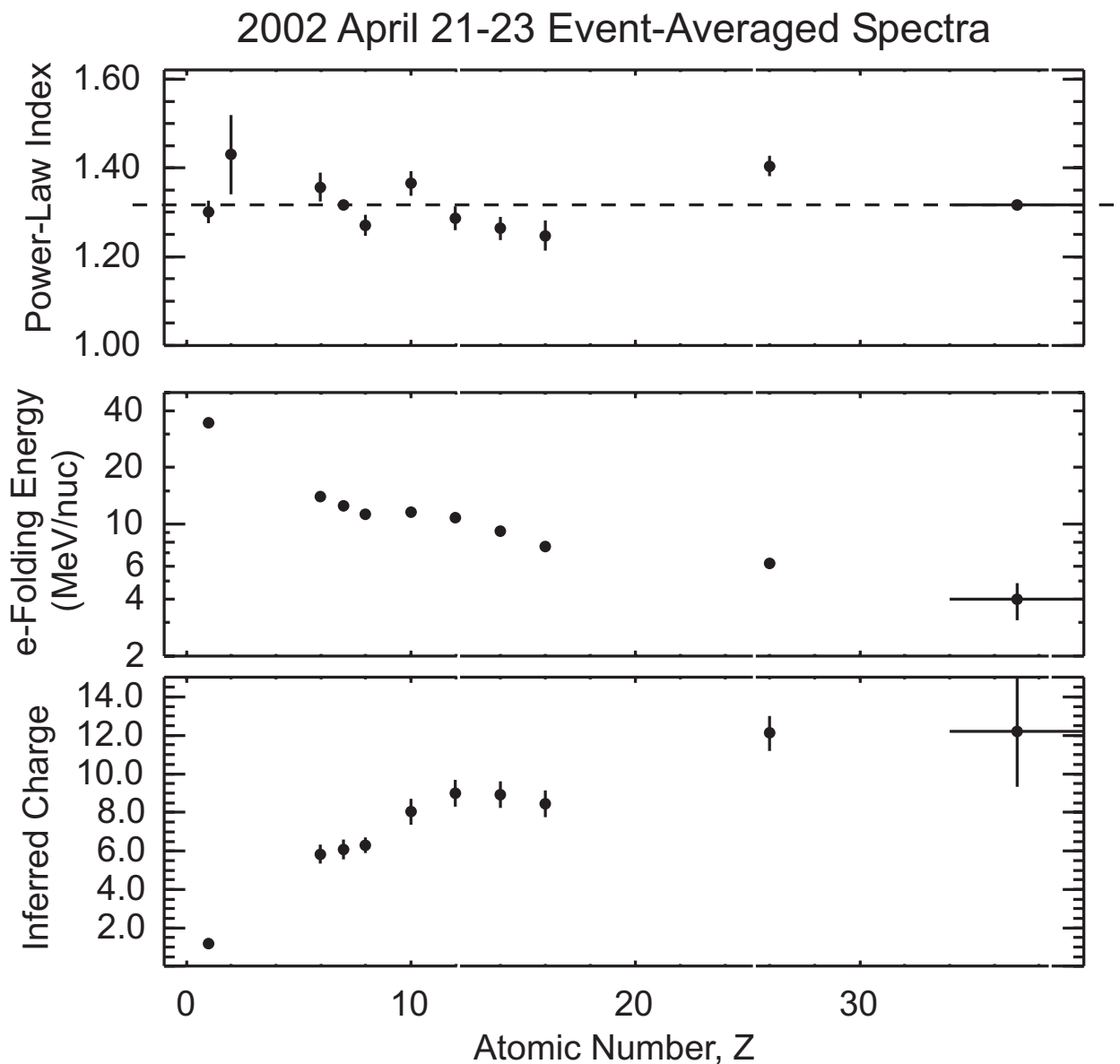
Fig. 8.— Fitted power-law indices (top), fitted e-folding energy (middle), and inferred mean ionic charge (bottom) plotted versus atomic number Z for event-averaged energy spectra in the 2002 April 21 event. The dashed line marks the weighted average of the datapoints in the top panel. For the fits to nitrogen and to ions at 34 \leq Z \leq 40 , the power-law index (top panel) has been fixed to the average value from the other species. In the bottom panel, the oxygen charge state measurement (from which the others are derived, as described in the text) came from SAMPEX (Labrador et al. 2003).
