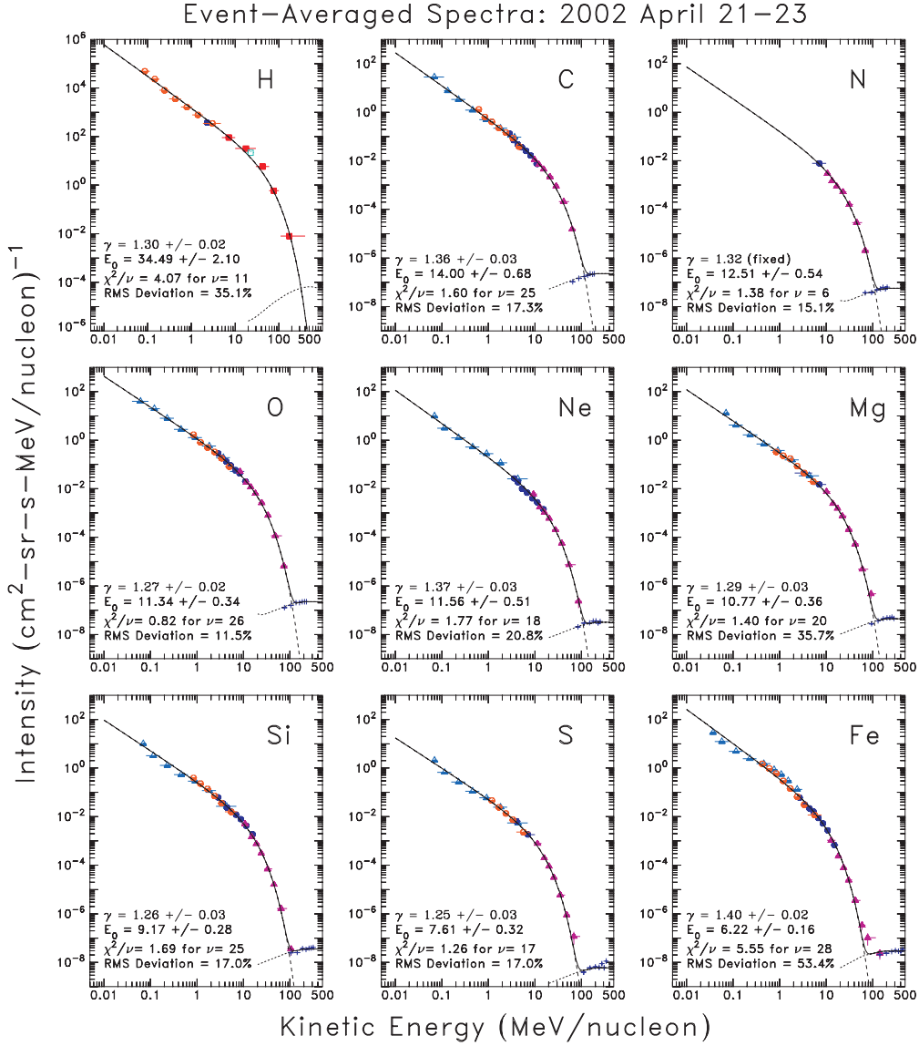
Fig. 7.— Event-averaged spectra for major elements in the 2002 April 21 solar particle event. The averaging interval began at 0:00 UT on 2002 April 21 and ended at 0:00 UT on 2002 April 24. Data are from ACE/ULEIS (light blue, half-filled triangles), ACE/EPAM (orange, half-filled circles), Wind/LEMT (dark blue, filled circles), ACE/SIS (purple, filled triangles), and GOES-8 (protons >5 MeV; red, filled squares). Blue crosses in the lower-right corners are Galactic cosmic ray (GCR) measurements from the Cosmic-Ray Isotope Spectrometer (CRIS; Stone et al. 1998b) on ACE . SEP intensities are fitted to the Ellison & Ramaty (1985) function (see text). Fit parameters, reduced \chi^2 , and rms deviation of the residuals are noted in each panel. For nitrogen, the power-law index has been fixed to the average value from the other species. In the lower-right corners, short dashes show estimated GCRs, and long dashes are the extrapolated SEP fits. Solid curves show the sum of fitted SEPs and GCRs.
