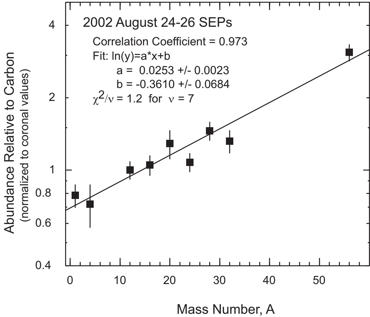
Fig. 16.— Elemental abundances relative to carbon (and normalized to nominal coronal values given by Reames (1995)) vs. mass number A for the 2002 August 24 SEP event. Also shown is an exponential fit to the correlation.
