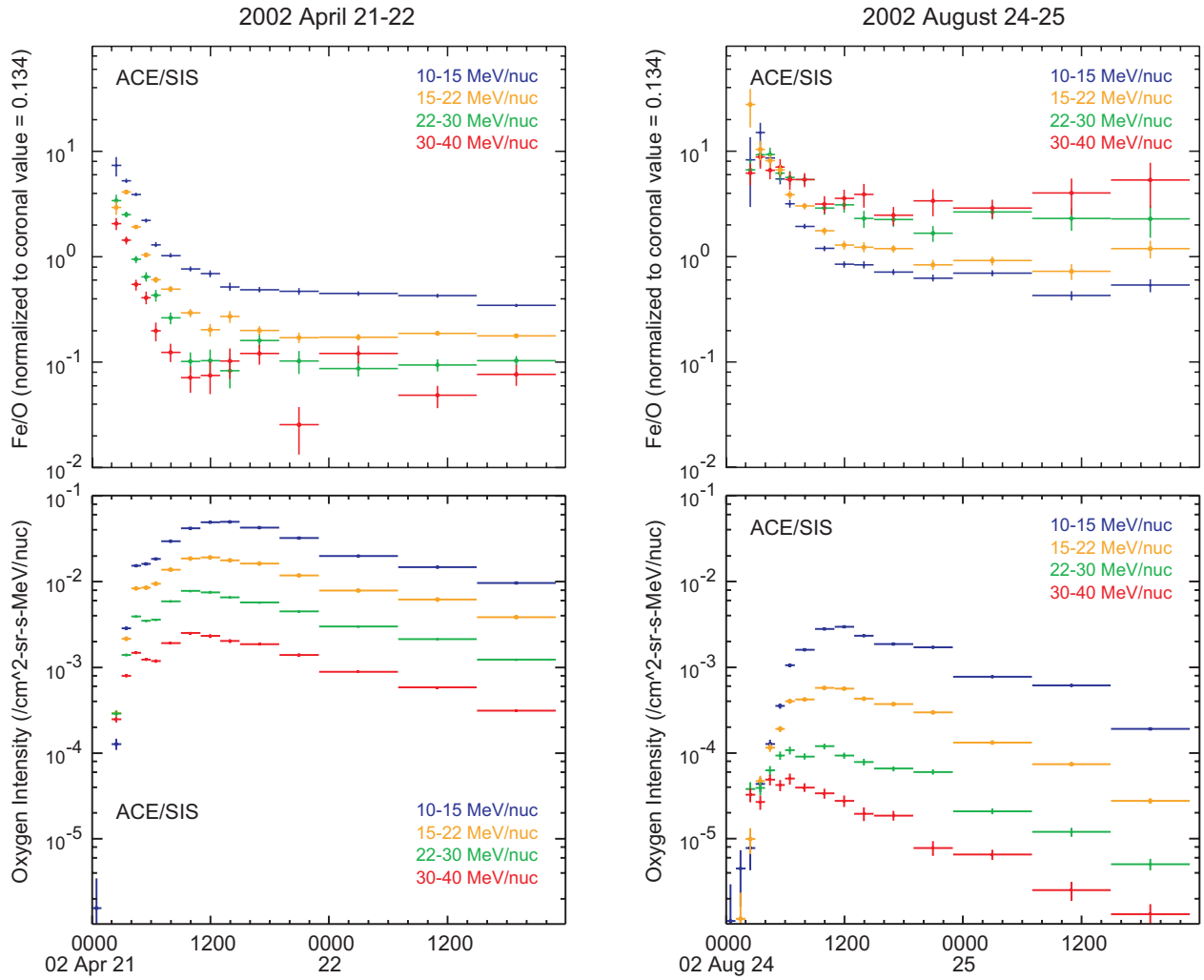
Fig. 5.— Fe/O (normalized to the nominal coronal value 0.134; top panels) and oxygen intensity (bottom panels) vs. time in the 2002 April 21 (left) and 2002 August 24 (right) events from ACE/SIS in four energy bins covering 10-40 MeV/nucleon, as distinguished by colors. Hourly-averages are shown in the first five hours of the event, but longer integration intervals are used later, when quantities are changing more slowly and/or ion statistics are smaller.
