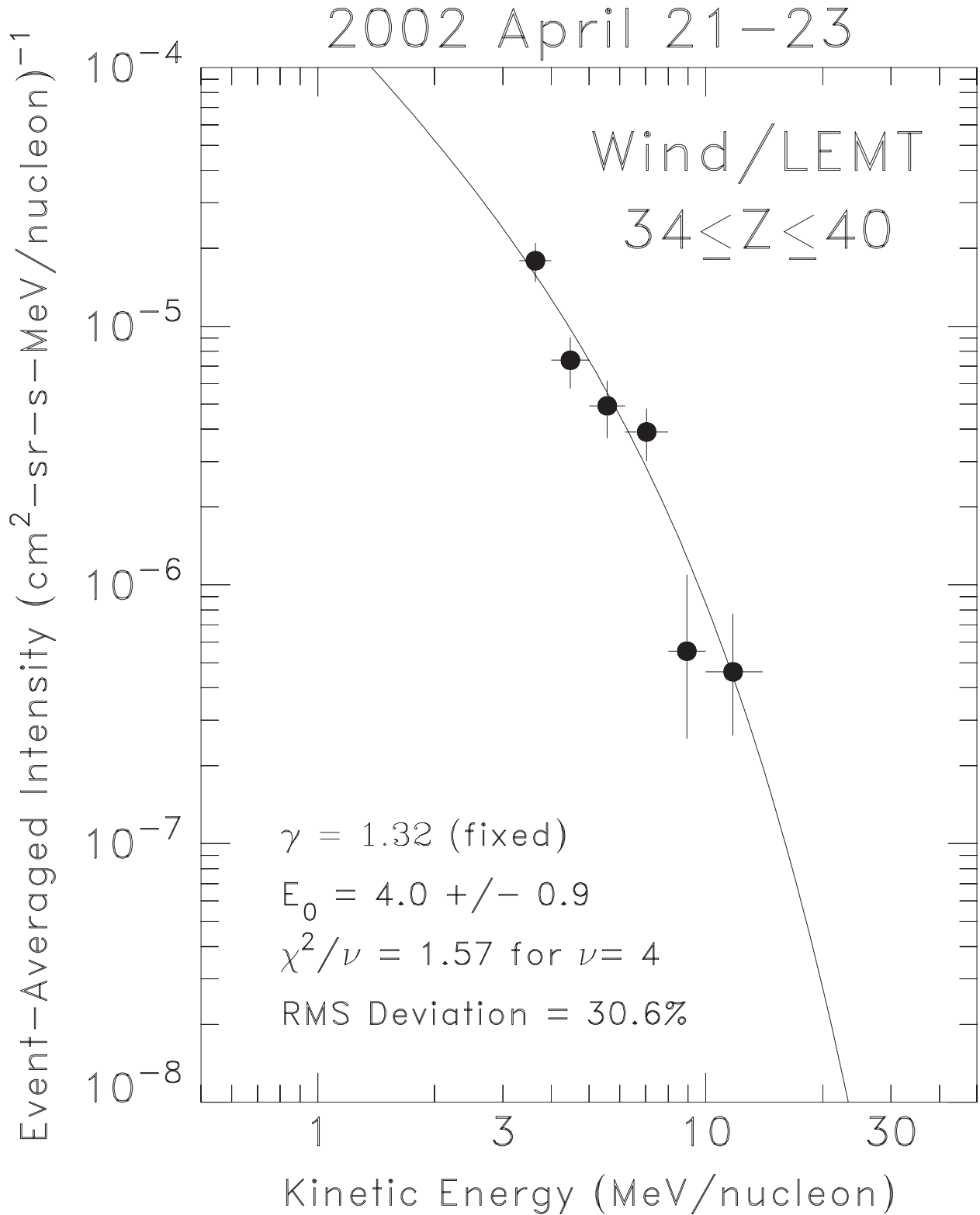
Fig. 9.— Event-averaged spectrum of ions with atomic number 34 \leq Z \leq 40 from Wind /LEMT in the 2002 April 21 event and its fitted Ellison & Ramaty spectrum, as described in the text. Datapoints are plotted with 1-sigma Poisson error bars (Gehrels 1986).
