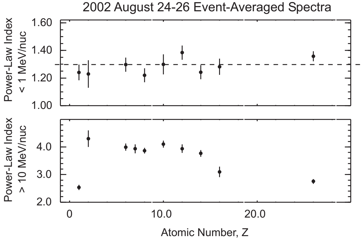
Fig. 14.— Fitted power-law indices below 1 MeV/nucleon (top) and above 10 MeV/nucleon (bottom) versus atomic number Z for event-averaged energy spectra in the 2002 August 24 event. The dashed line marks the weighted mean of the datapoints in the top panel.
