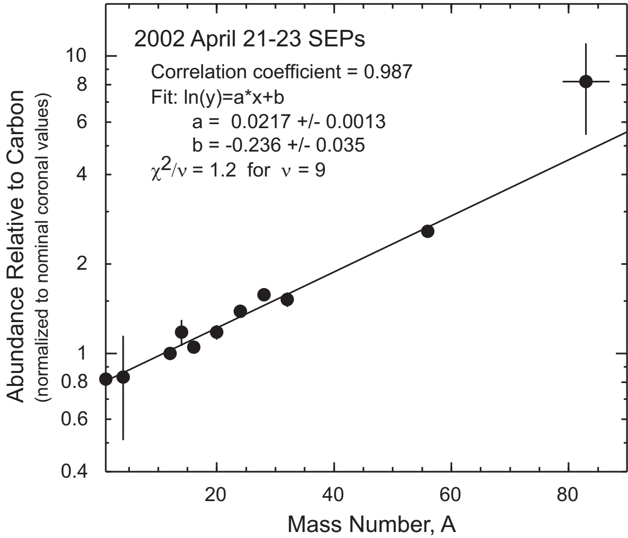
Fig. 12.— Elemental abundances relative to carbon (and normalized to nominal coronal values given by Reames (1995; 2000)) vs. mass number A for the 2002 April 21 SEP event. Also shown is an exponential fit to the correlation.
