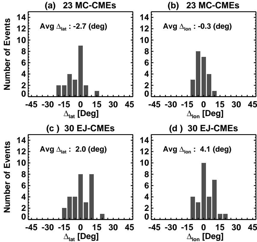
Figure 6. Histograms of latitudinal difference between the CME source locations and propagation directions \Delta_{lat} for a) 23 MC-CMEs and c) 30 EJ-CMEs, and histograms of longitudinal difference \Delta_{lon} for b) 23 MC-CMEs and d) 30 EJ-CMEs.
