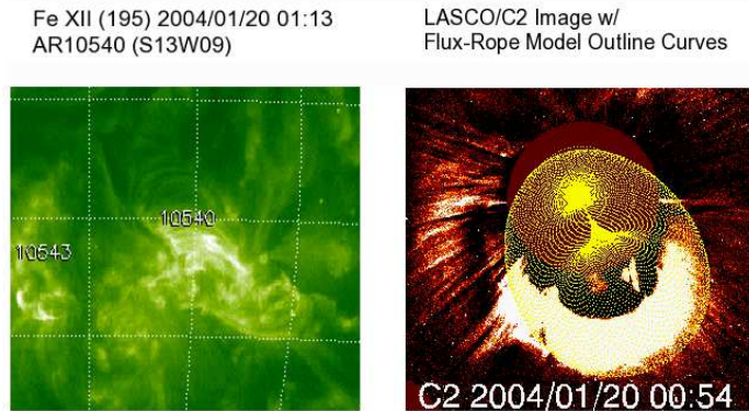
Figure 2. An example of the flux-rope model fit for the 2004 January 20 CME. (Left) EIT 195 Å image showing the flare post-eruption arcade at 01:13 UT. (Right) LASCO/C2 image at 00:54 UT superimposed with the flux-rope model outline curves (yellow curves).
