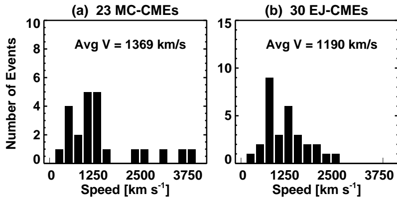
Figure 8. Histograms of KFR-fit radial speed V_{cme} for a) 23 MC-CMEs and b) 30 EJ-CMEs.
