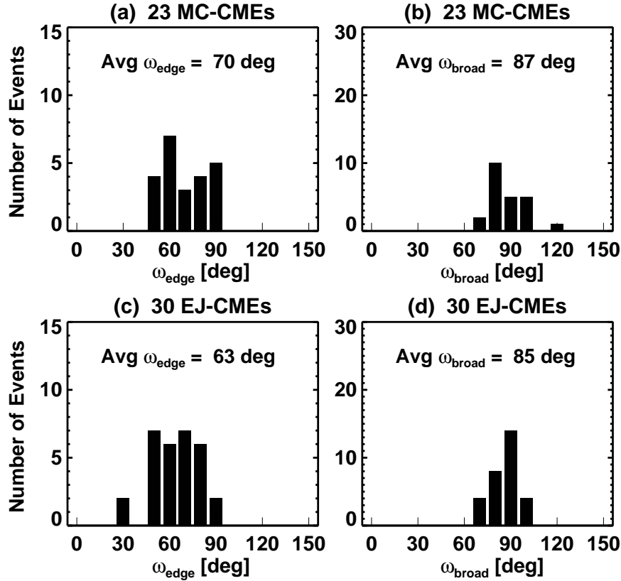
Figure 7. Histograms of KFR-fit widths: a) edge-on width \omega_{edge} and b) broadside width \omega_{broad} for 23 MC-CMEs, c) \omega_{edge} and d) \omega_{broad} for 30 EJ-CMEs.
